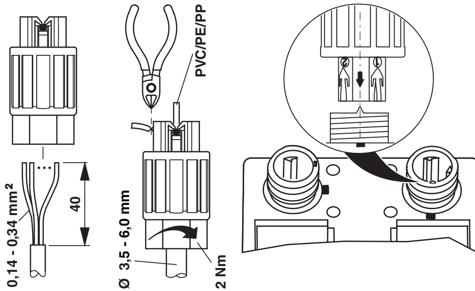
Functional drawing
